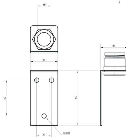
Wall mounting device for sensor
